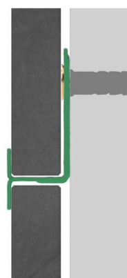
Grapa Intermedia (visible)
